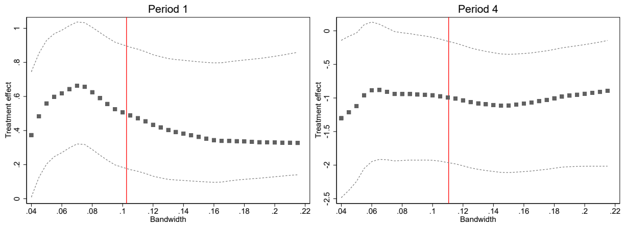
Figure D3: Impact on COVID-19 deaths: Robustness to bandwidth choice
